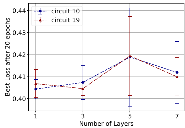
(b) Number of layers ( N_L ) comparison.
